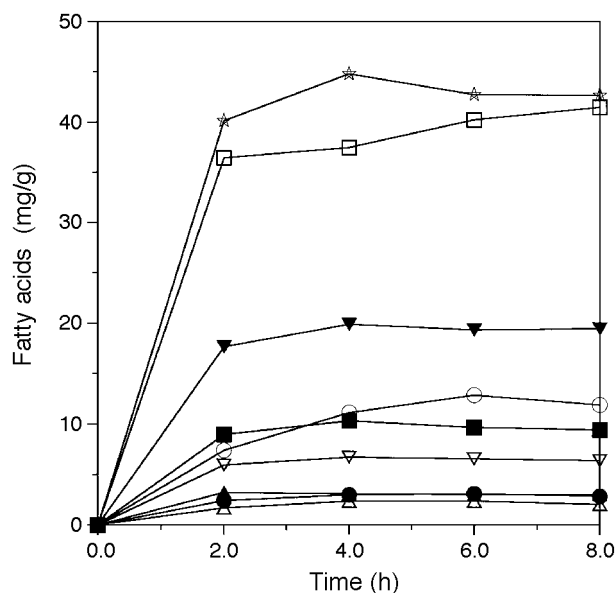
FIG. 1. Free fatty acid concentration as a function of time during hydrolysis of the short-chain butterfat fraction: \circ , C_{4:0} ; \bullet , C_{6:0} ; \triangle , C_{8:0} ; \blacktriangle , C_{10:0} ; \nabla , C_{12:0} ; \blacktriangledown , C_{14:0} ; \square , C_{16:0} ; \blacksquare , C_{18:0} ; \star , C_{18:1} .
