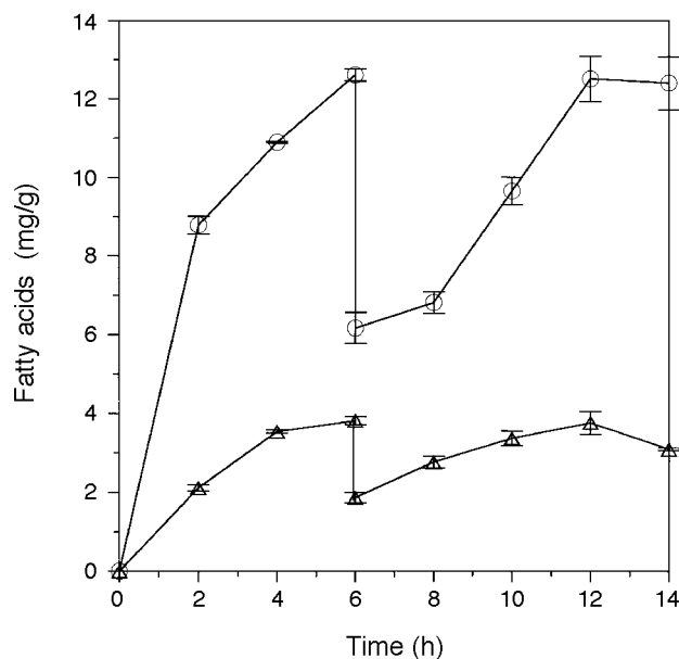
FIG. 2. Free fatty acid concentration as a function of time during hydrolysis of the short chain butterfat fraction with dilution after 6 h: \circ , C_{4:0} ; \triangle , C_{8:0} .
